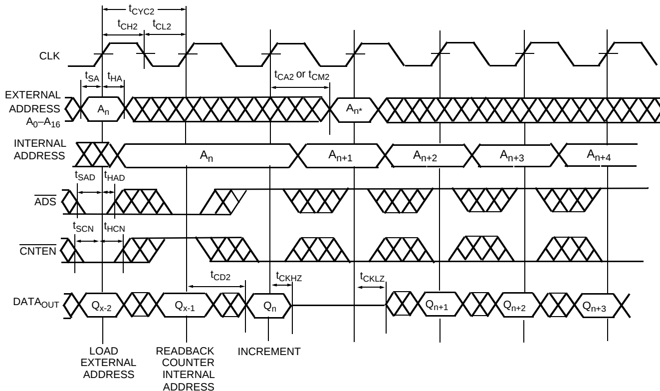
Figure 20. Readback State of Address Counter or Mask Register [51, 52, 53, 54]
