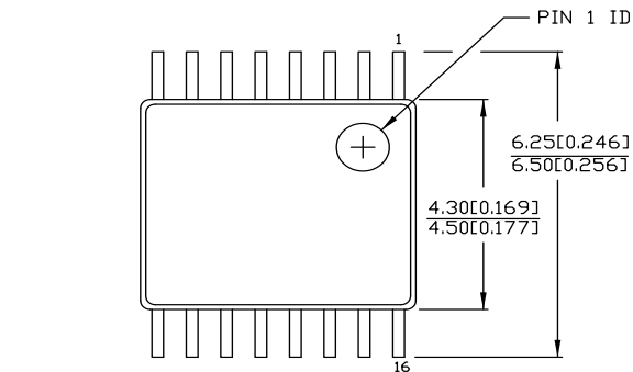
Figure 13. 16-Pin TSSOP (4.40 mm Body) Package Outline, 51-85091
