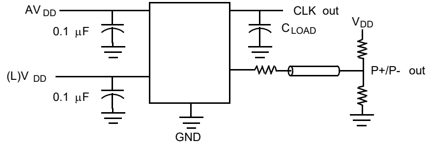
Figure 12. Test Circuit
