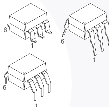
Figure 1. Package Outlines
