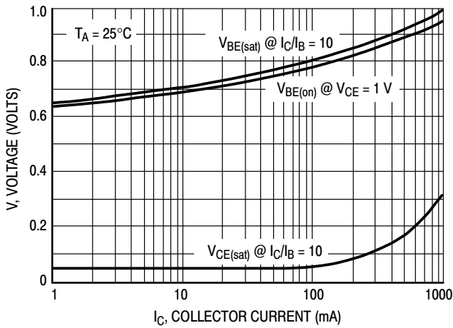
Figure 3. "On" Voltages
