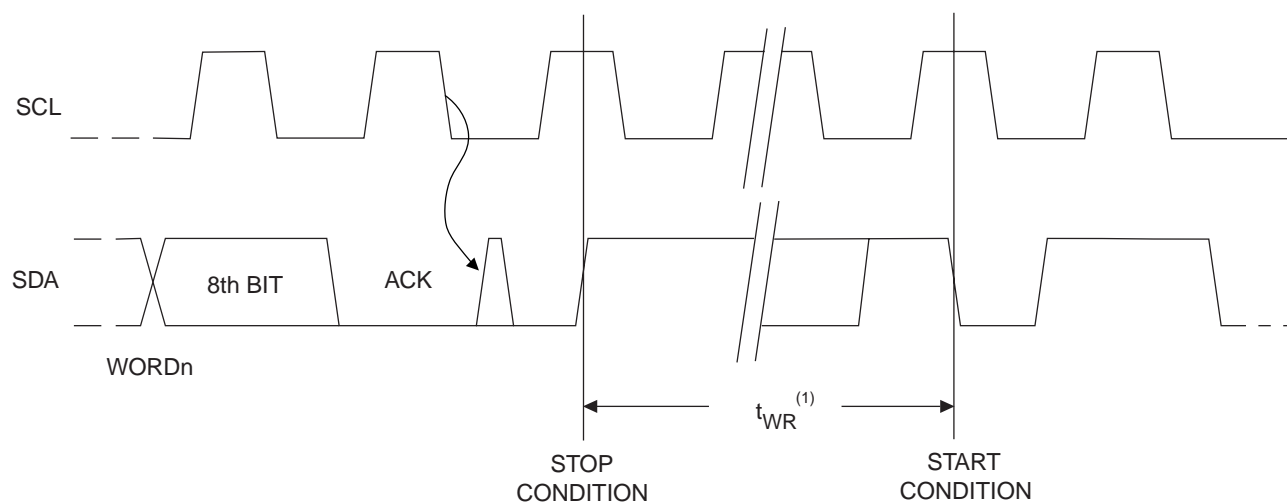
Figure 11-2. Write Cycle Timing
