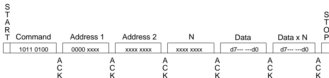
Figure 7-9. System Write
