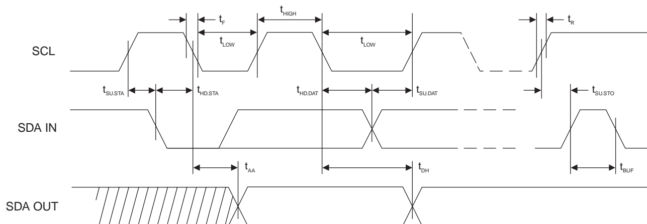
Figure 11-1. Bus Timing
