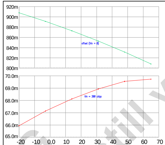
Figure 7. RSSI-step [V] @ V_{in} = 300\text{ }\mu\text{Vpp} and offset vs. temp [deg C], reduced step
