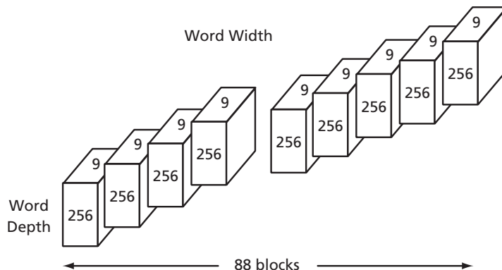
Figure 1-23 • APA1000 Memory Block Architecture
