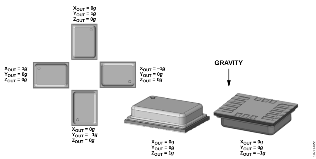
Figure 64. Output Response vs. Orientation to Gravity
