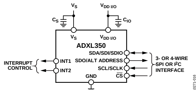
Figure 58. Application Diagram
