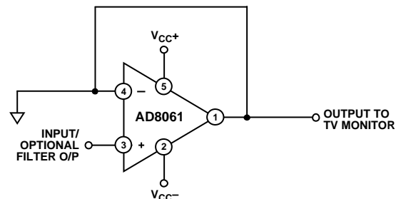
Figure 82. Recommended Output DAC Buffer
