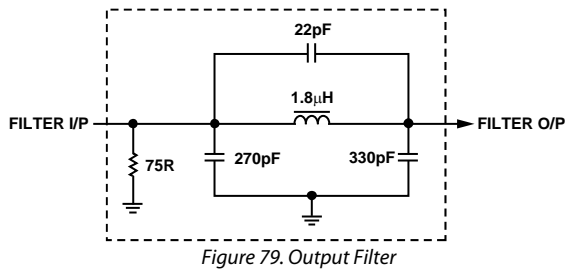
Figure 79. Output Filter
