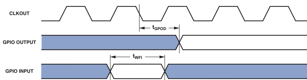
Figure 26. General-Purpose Port Timing
