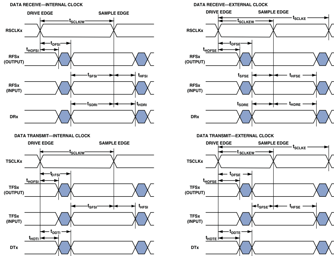
Figure 20. Serial Ports
