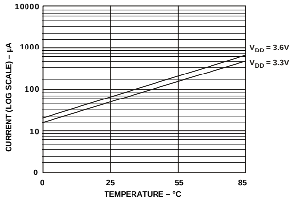
Figure 37. Typical Power-Down Current (ADSP-2185L)
