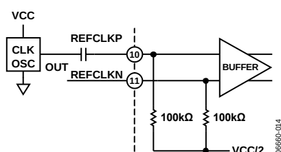
Figure 16. Single-Ended REFCLK Configuration
