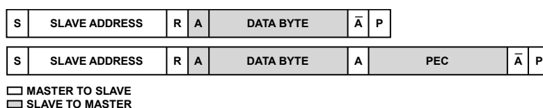
Figure 57. Receive Byte and Receive Byte with PEC
