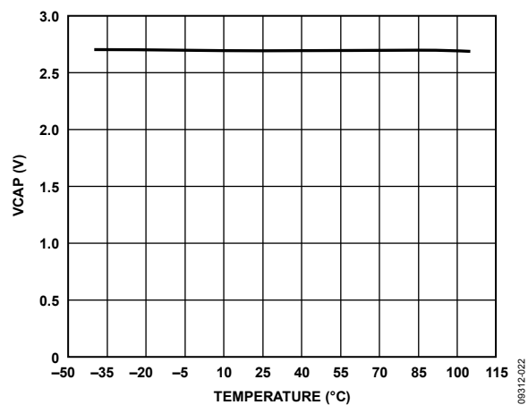
Figure 22. V_{\text{CAP}} vs. Temperature ( I_{V_{\text{CAP}}} = 100 \mu\text{A} )
