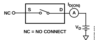
Figure 22. Drain Off Leakage
