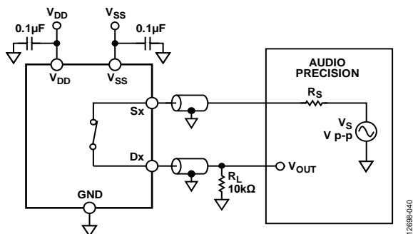
Figure 41. THD + N
