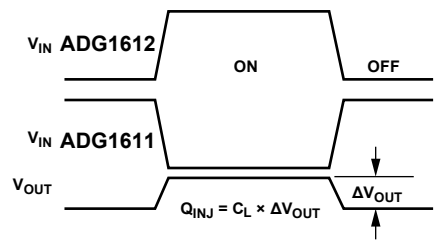
Figure 33. Charge Injection
