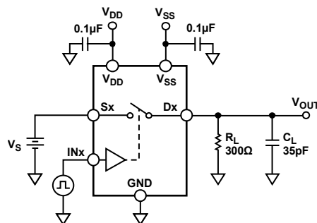
Figure 31. Switching Times
