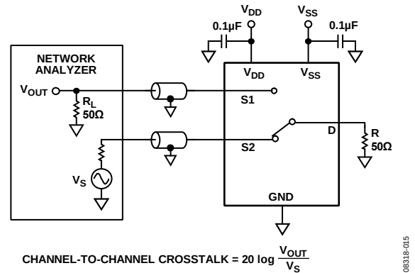
Figure 34. Channel-to-Channel Crosstalk
