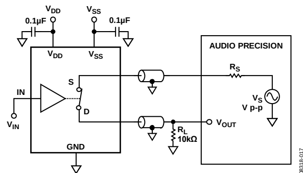
Figure 35. THD + Noise
