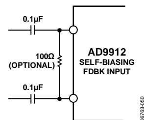
Figure 38. FDBK_IN Input
