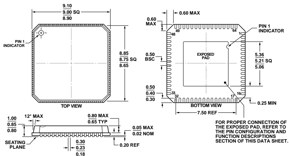
Figure 57. 64-Lead Lead Frame Chip Scale Package [LFCSP_VQ] 9 mm x 9 mm Body, Very Thin Quad (CP-64-7)
