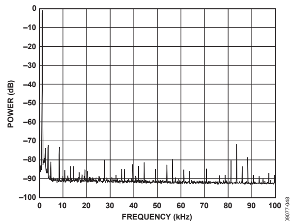
Figure 16. Power vs. Frequency, f_{CLK} = 5\text{ MHz} , f_{OUT} = 1.2\text{ kHz} , Frequency Word = 0x000FBA9
