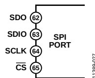
Figure 36. SPI Pins
