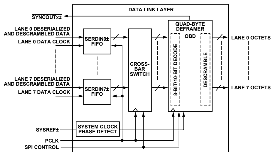
Figure 98. Data Link Layer Block Diagram
