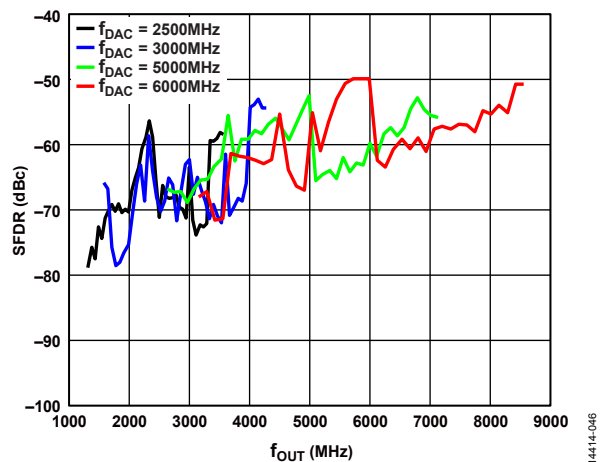
Figure 50. SFDR vs. f_{OUT} over f_{DAC}
