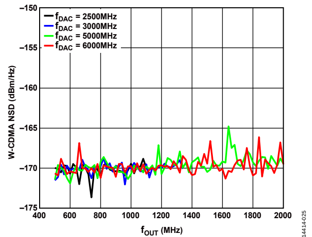
Figure 27. W-CDMA NSD Measured at 70 MHz vs. f_{OUT} over f_{DAC}
