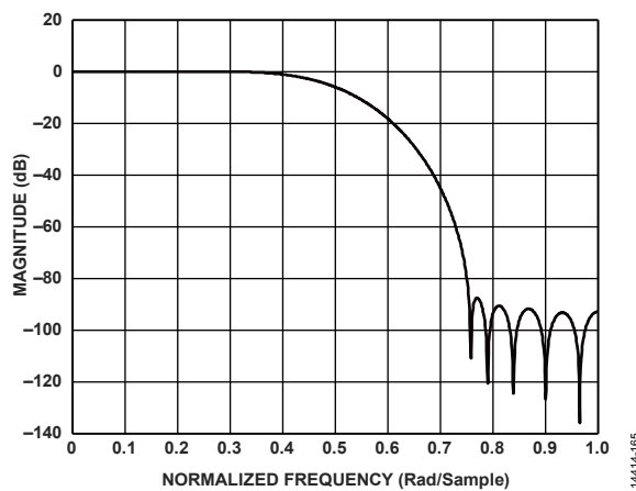
Figure 119. FIR85 2x Half-Band 45% Filter Response
