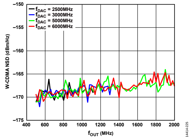
Figure 28. W-CDMA NSD Measured at 10% Offset from f_{OUT} vs. f_{OUT} over f_{DAC}
