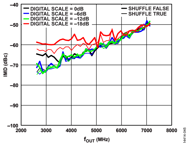
Figure 49. IMD vs. f_{OUT} over Digital Scale
