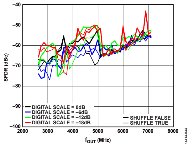
Figure 48. SFDR vs. f_{OUT} over Digital Scale
