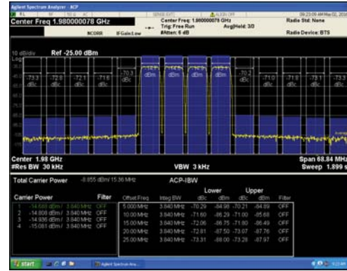
Figure 57. Four-Carrier W-CDMA at 1980 MHz
