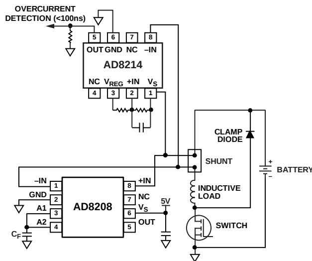
Figure 27. Battery-Referenced Shunt Resistor
