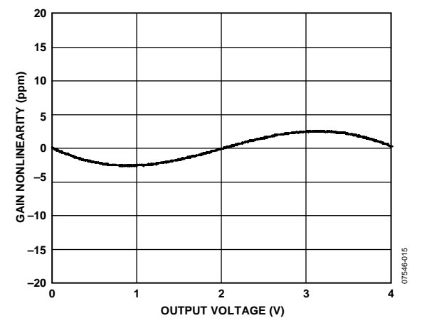
Figure 16. Gain Nonlinearity, R_L = 600\ \Omega , 2 k \Omega , 10 k \Omega
