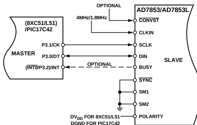
Figure 45. 8XC51/PIC17C42 Interface
