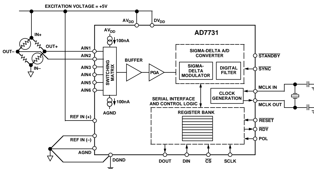
Figure 22. Pressure Measurement Using the AD7731
