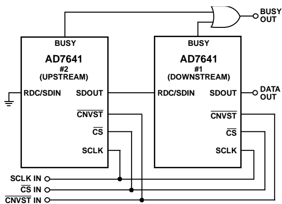
Figure 38. Two AD7641 Devices in a Daisy-Chain Configuration
