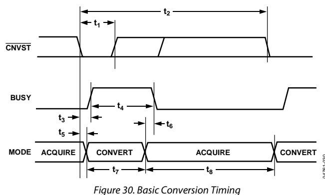
Figure 30. Basic Conversion Timing
