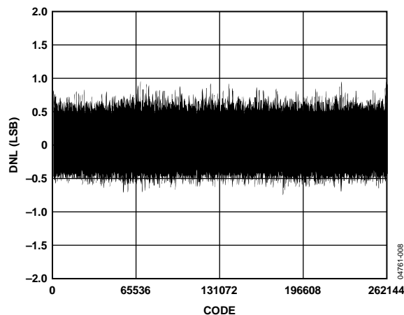
Figure 9. Differential Nonlinearity vs. Code
