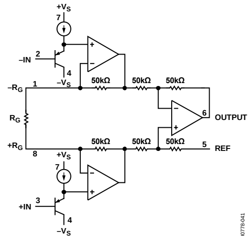
Figure 70. Simplified Schematic
