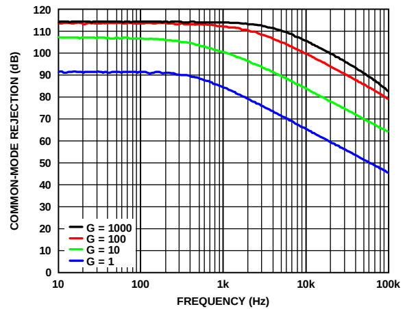
Figure 25. Common-Mode Rejection vs. Frequency, +V_S = 5 V, -V_S = 0 V, V_{REF} = 2.5 V, for Various Gain Settings, RM-8 and R-8 Package Options
