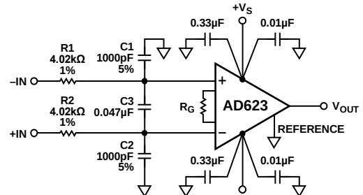
Figure 74. Circuit to Attenuate RF Interference
