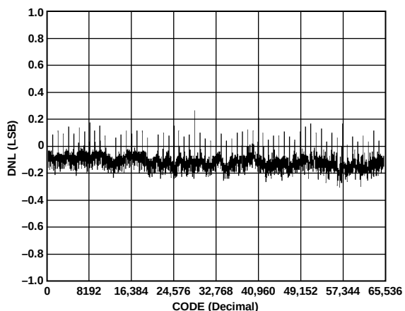
Figure 8. AD5543 DNL Error
