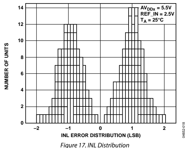
Figure 17. INL Distribution
