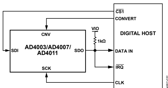
Figure 63. \overline{\text{CS}} Mode, 4-Wire with Busy Indicator Connection Diagram
