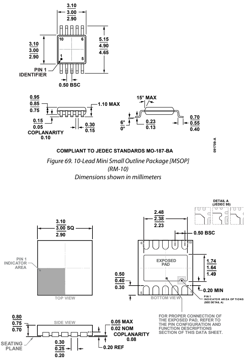
Figure 70. 10-Lead Lead Frame Chip Scale Package [LFCSP] 3 mm × 3 mm Body and 0.75 mm Package Height (CP-10-9)
