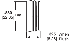
Side View Plugs/Receptacles
