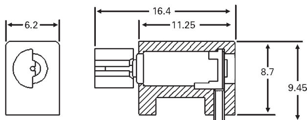
VIB MOTOR CONNECTOR ASSEMBLY
