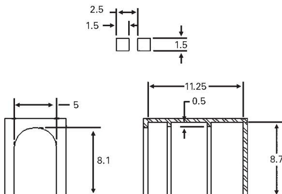
RECOMMENDED APPLICATION HOUSING SIZE
