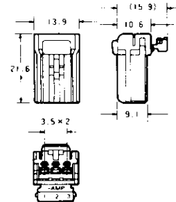
Plug (Mark I/Mark II)
