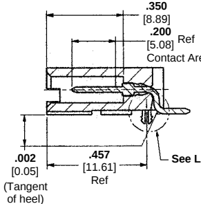
Section K-K
