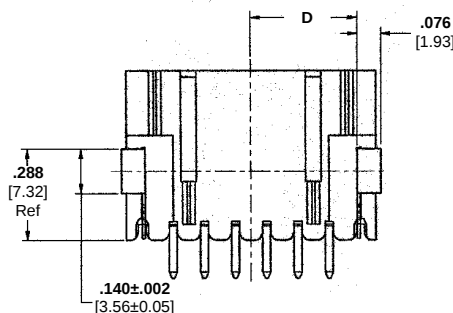
Section K-K
