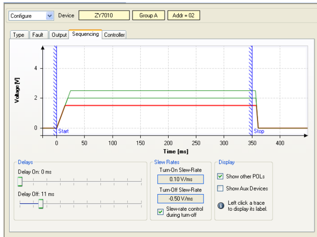
Figure 32. POL Configure Sequencing Window
