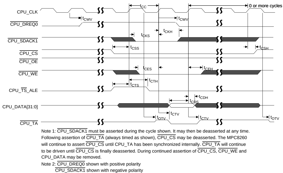
Figure 46 - CPU DMA Write - MPC8260
