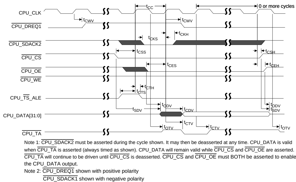
Figure 45 - CPU DMA Read - MPC8260
