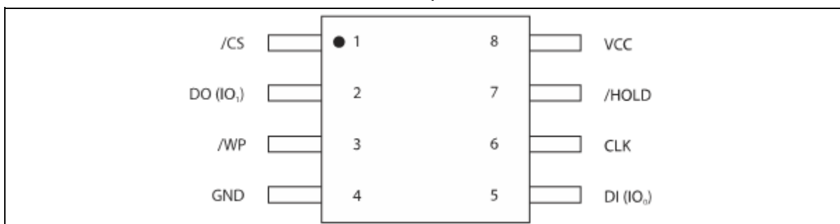
Figure 1a. W25X20CL Pin Assignments, 8-pin SOIC 150-mil, AND VSOP 150-mil (Package Code SN, AND SV)
