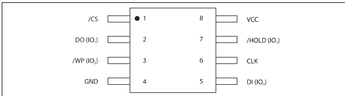
Figure 1a.W25Q20EW Pin Assignments, 8-pin SOIC 150-mil and VSOP 150-mil (Package Code SN & SV)
