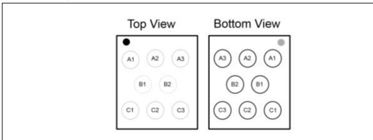
Figure 1c. W25Q20EW Ball Assignments, 8-ball WLCSP (Package Code BY)
