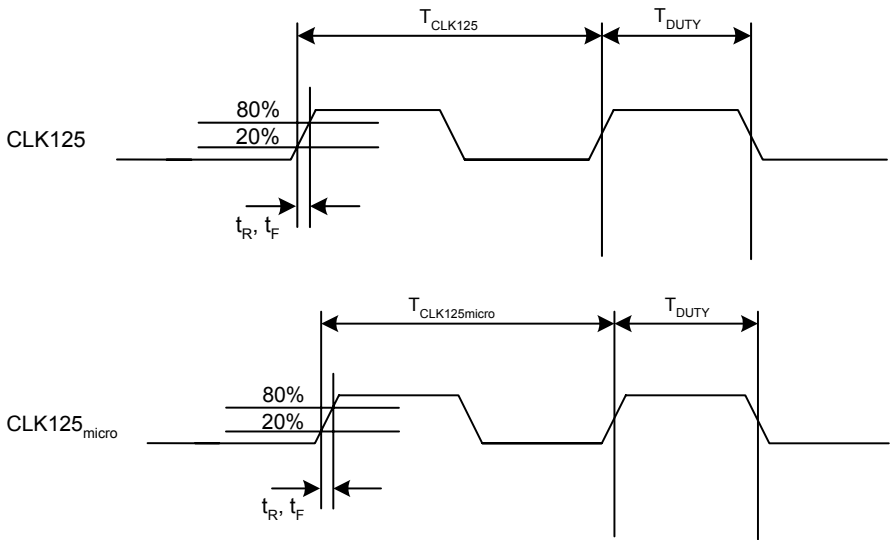
Figure 35. CLK125 AC Timing
