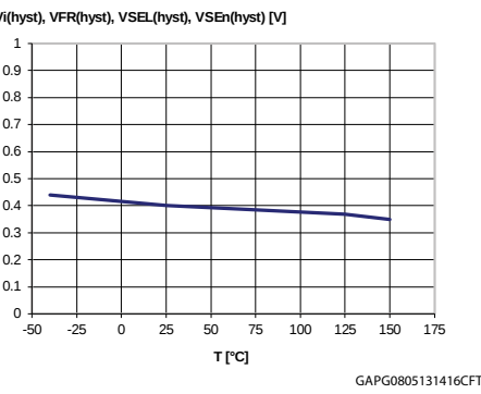
Figure 22: Logic Input hysteresis voltage
