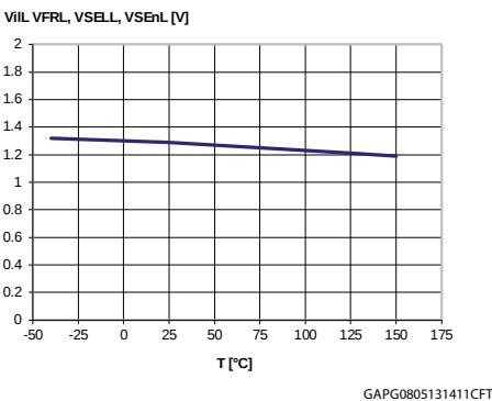
Figure 19: Logic Input low level voltage
