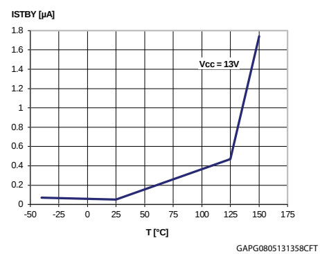
Figure 16: Standby current
