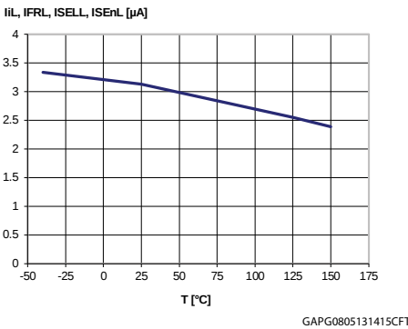
Figure 21: Low level logic input current
