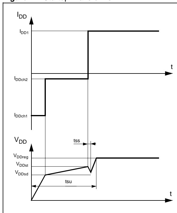
Figure 17: Startup Waveforms
