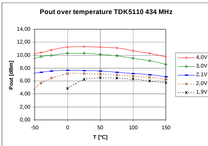
Figure 4-4 Pout over temperature of the 50Ω-testboard with TDK5110 at 434 MHz
