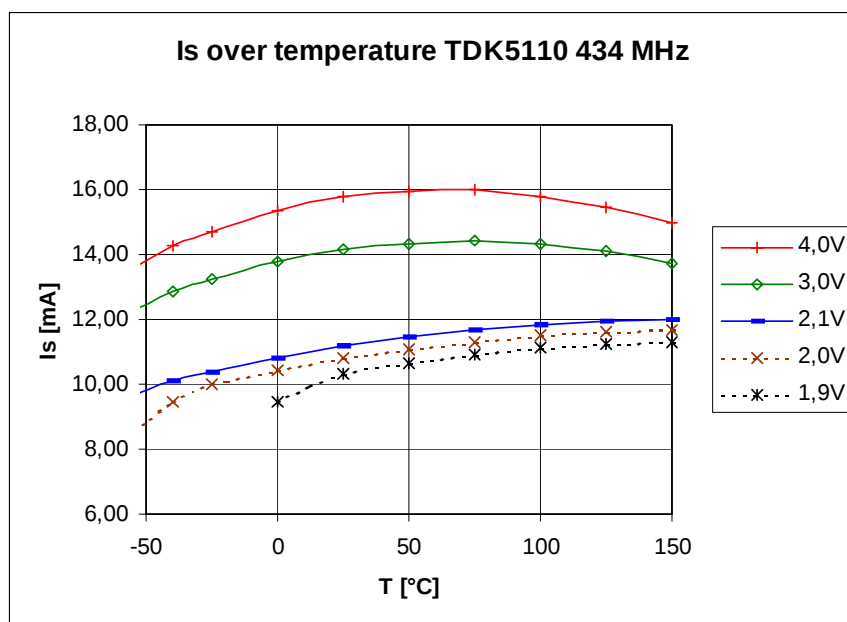
Figure 4-5 Is over temperature of the 50Ω-testboard with TDK5110 at 434 MHz
