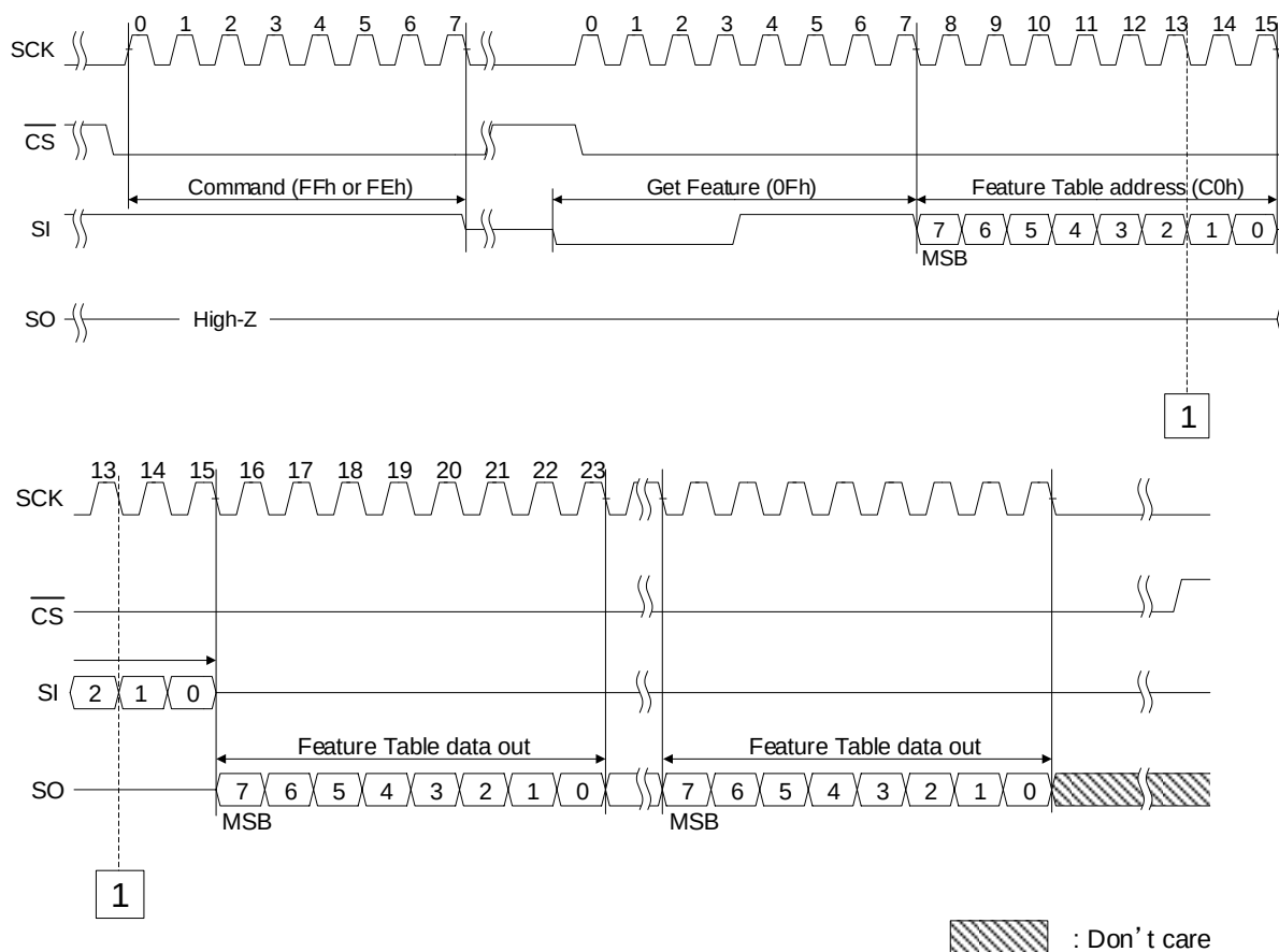
Figure 19. Reset Timing
