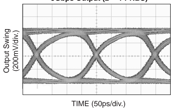
5Gbps Output ( 2^{23}-1 PRBS)
