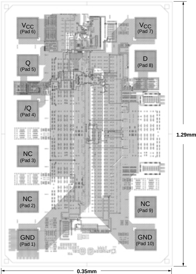
Figure 1. Chip Topography
