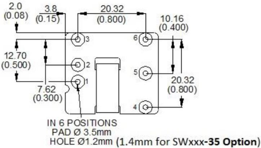
Through-Hole Pad Layout – Component side view
