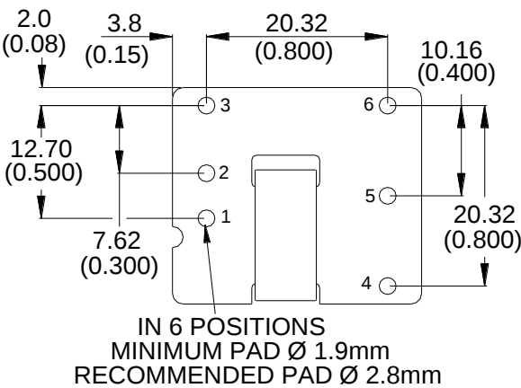
Surface Mount Pad Layout – Component side view
