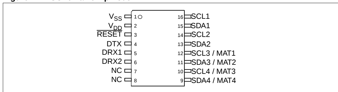
Figure 2. SO16 narrow pinout
