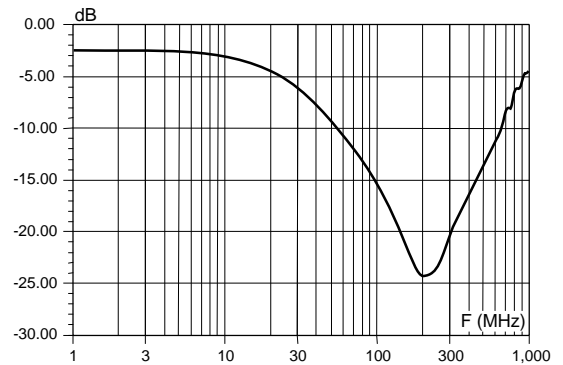
Figure 6: Typical frequency response curve for data and STROBE signal
