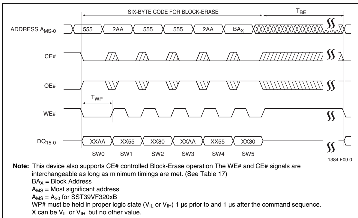
Figure 11: WE# Controlled Block-Erase Timing Diagram
