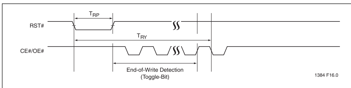
Figure 18: RST# Timing Diagram (During Program or Erase operation)
