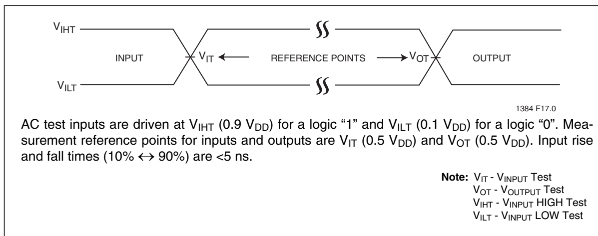
Figure 19: AC Input/Output Reference Waveforms
