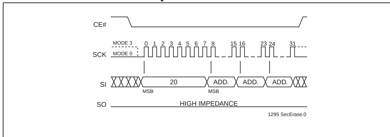
FIGURE 4-10: SECTOR-ERASE SEQUENCE
