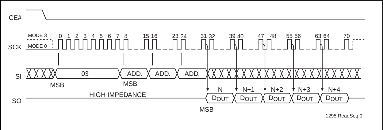
FIGURE 4-3: READ SEQUENCE
