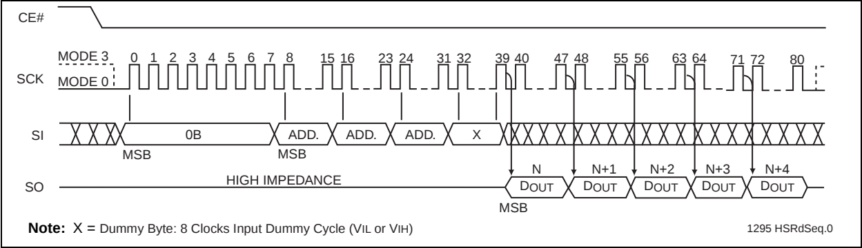
FIGURE 4-4: HIGH-SPEED-READ SEQUENCE
